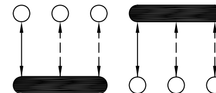
SCHEMATIC (SHORTING)
